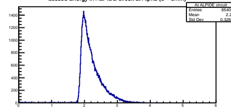
Lossed Energy in ALPIDE circuit at Alpha (d = 9mm)
